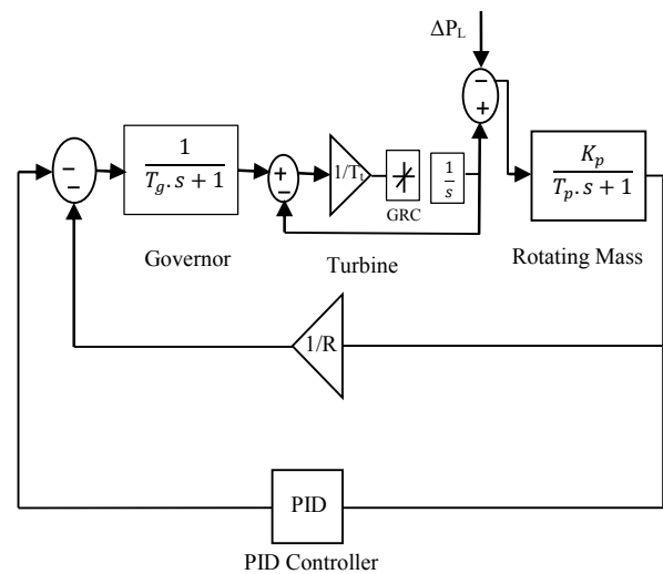
Fig.6. Simulink model under study for case 2
