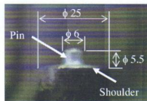
Fig. 2. H13 FSW tool.
