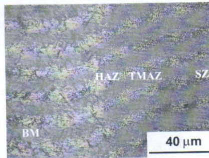
Fig. 6. Microstructure of FSW joint at the advancing side of the WZ edge ( \omega = 800 rpm and v = 12 mm/min).
