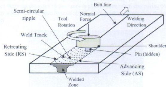
Fig. 1. A schematic description of FSW process.
