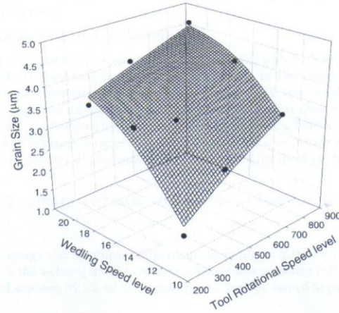
Fig. 8. Variation of \alpha -Al grain size with both tool rotation and welding speeds.
