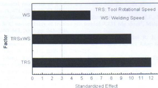
Fig. 11. Standardized Pareto chart for size of Si particulates.
