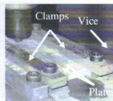
Fig. 3. Plates fixation during FSW.
