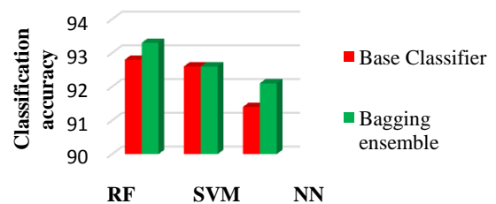
Figure 4. The improvement in overall classification accuracy at using BE with RF, SVM and NN base classifiers.
